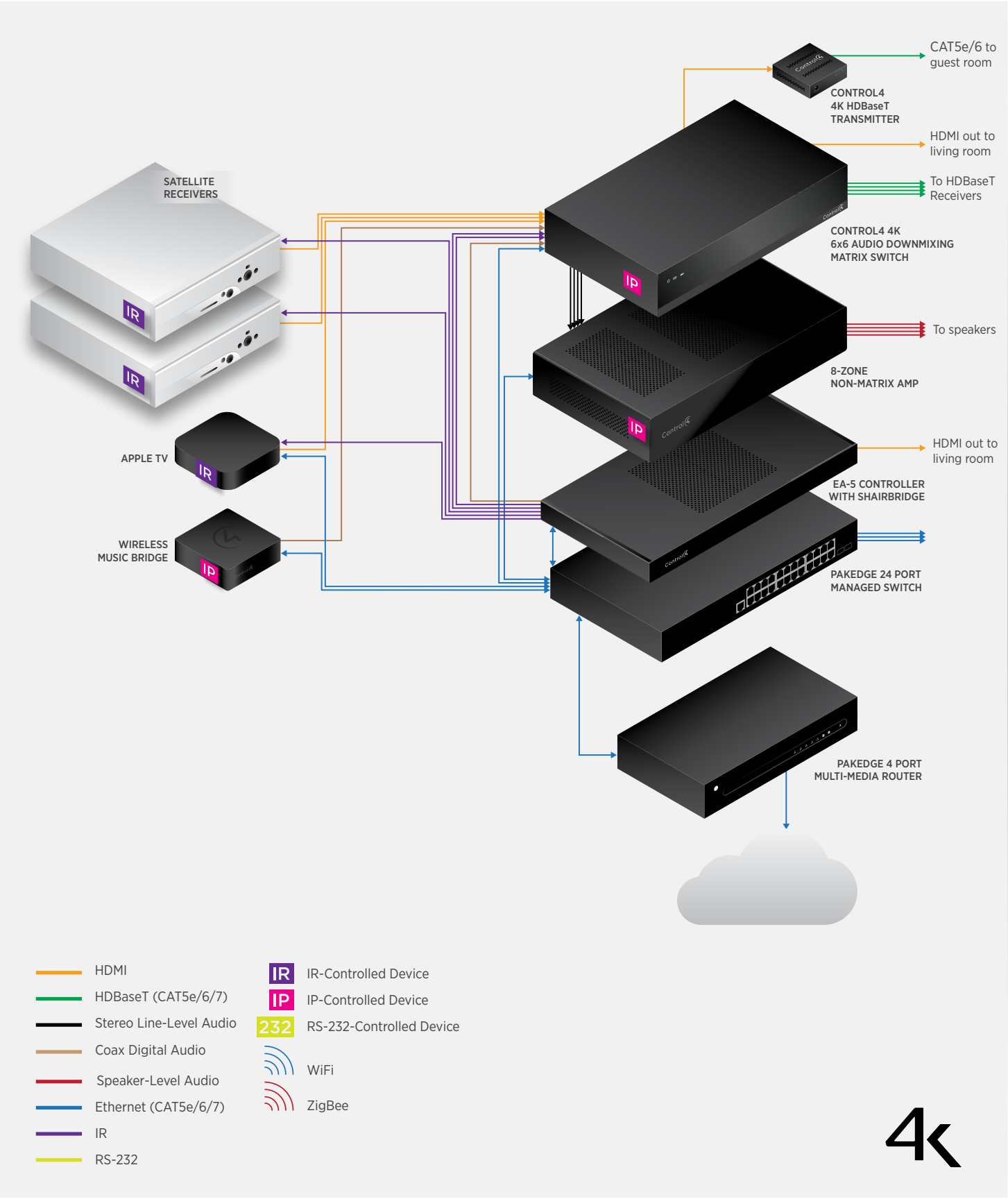
Living Room Equipment Rack
